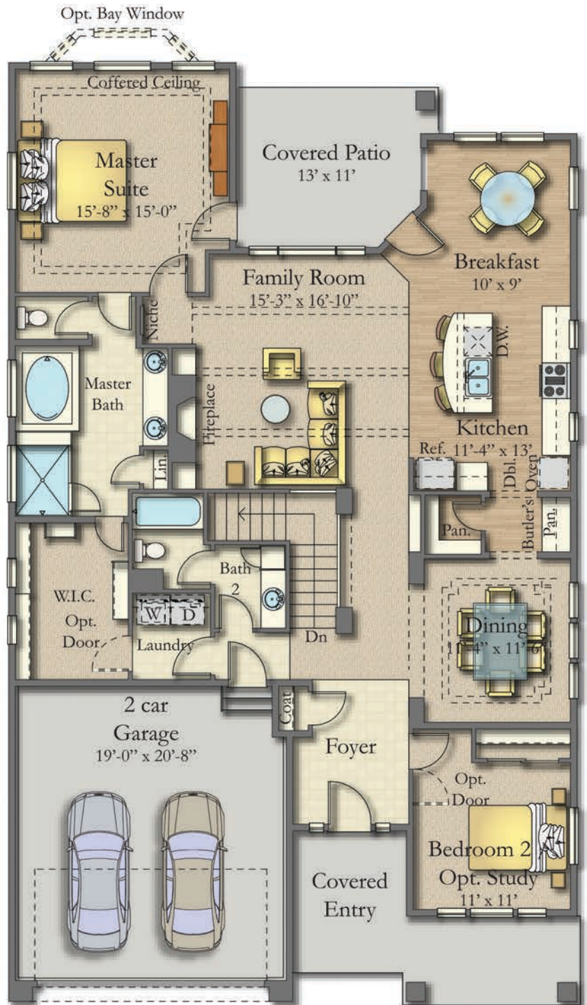
MAIN LEVEL 1,803 SQ.FT.
